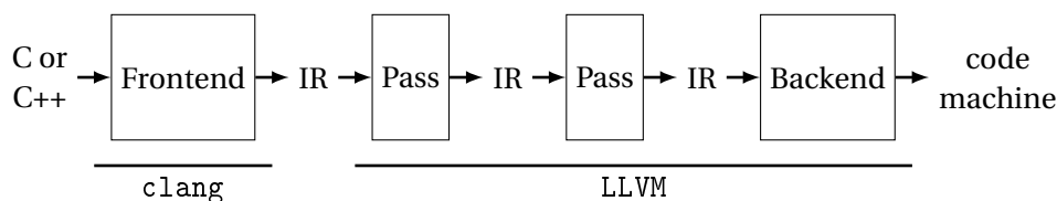
FIGURE 1 – L'infrastructure clang-LLVM
